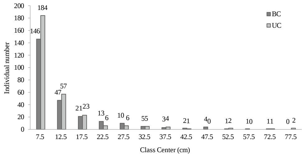
Fig. 3 Diameter distribution of trees in the forest formations in RPPN BF, Burnt Forest and UF, Unburnt Forest
